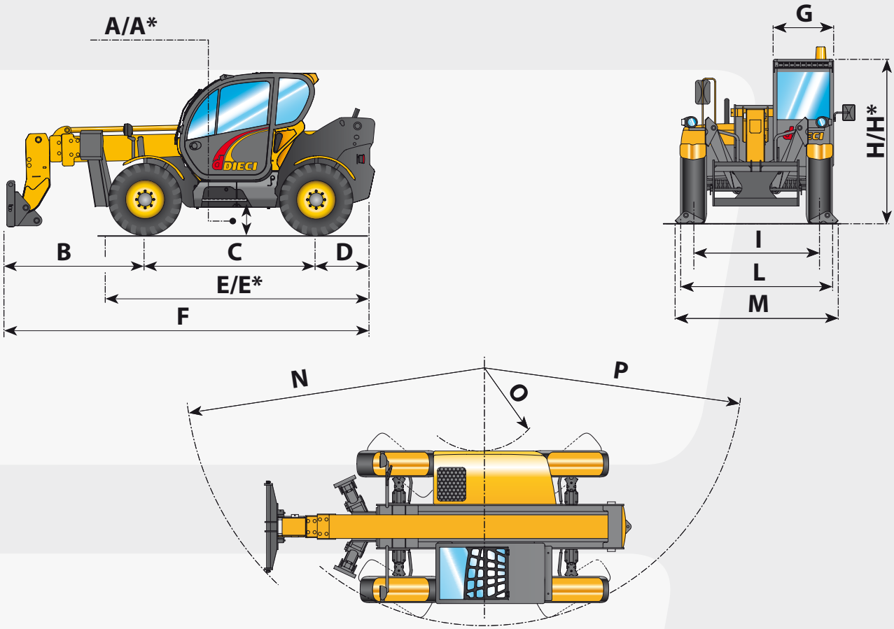
A* - E* - H* = Measurements referring to optional wheels
