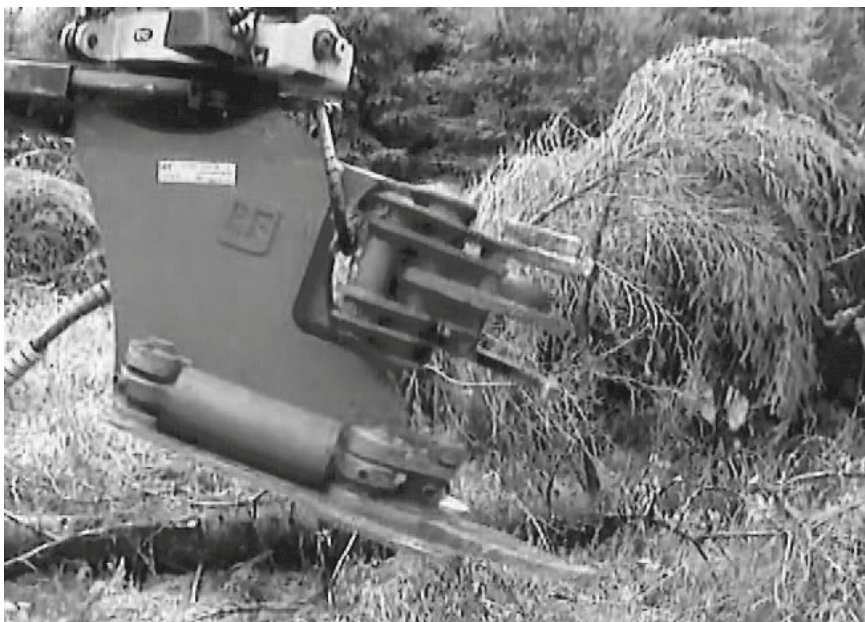
Tree Cutter TKL 22 with intergated gripper
